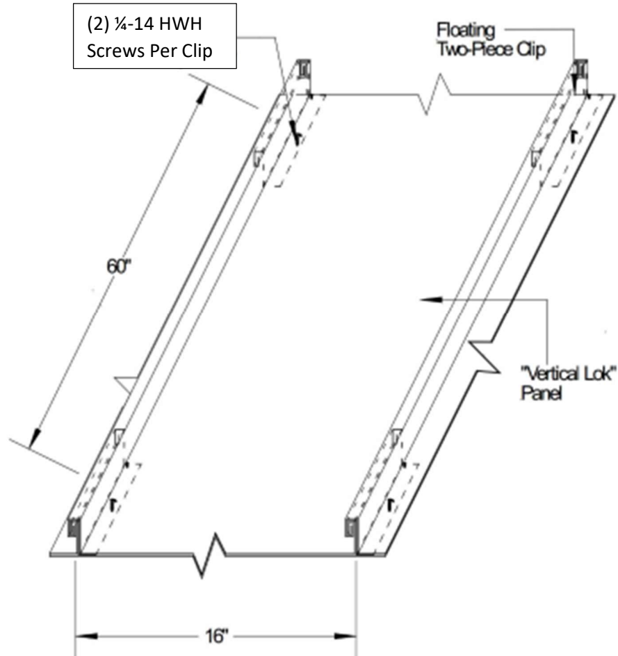
Typical Roof Assembly Isometric View
