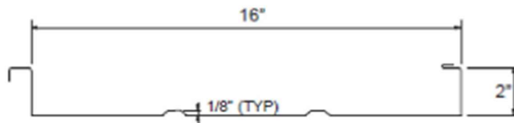
Typical Panel Profile
